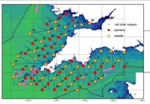
Fig: map of the different stations during the survey 22/17
