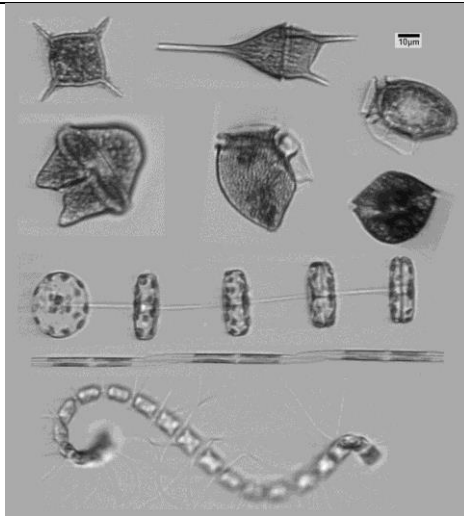
Phytoplankton images acquired using the Imaging FlowCytobot
